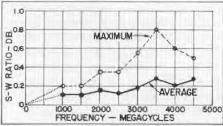
Figure 5. Type 874 Connector standing-wave ratio as a function of frequency.
