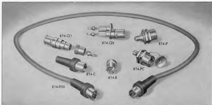
Figure 8. Coaxial connectors and parts now available.
